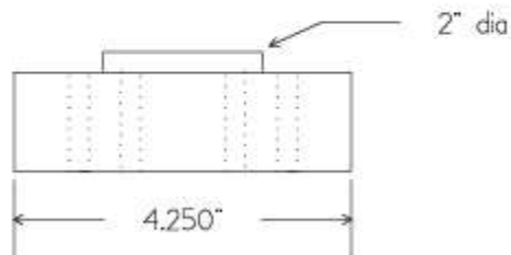
Detail of drill guide
